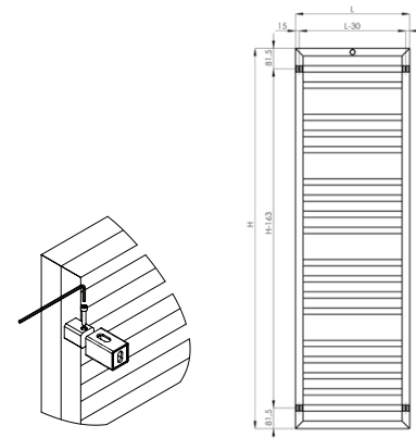
CHAUFFAGE CENTRAL
